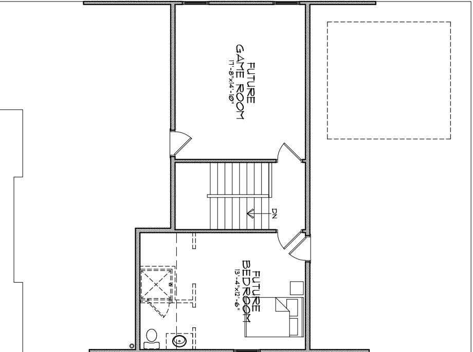
OPTIONAL ATTIC FLOOR PLAN
